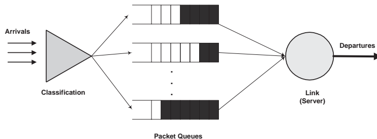
Figure 1: Queuing Model
